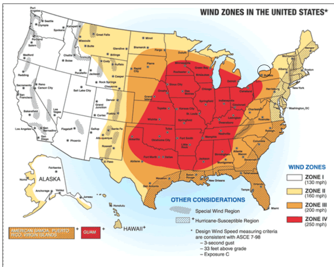
Figure 14-1. Wind Zones in the United States
